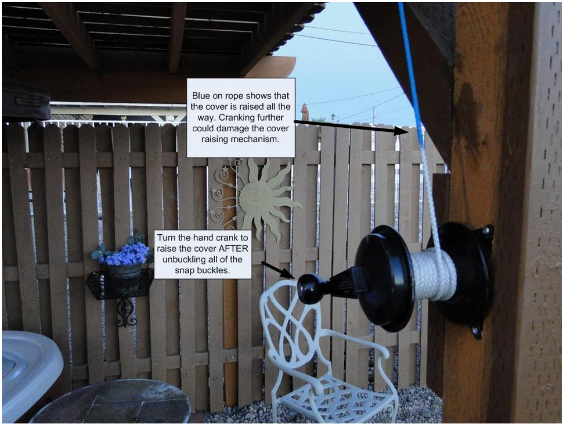
Figure 4. The hand crank is used to raise and lower the hot tub cover.
