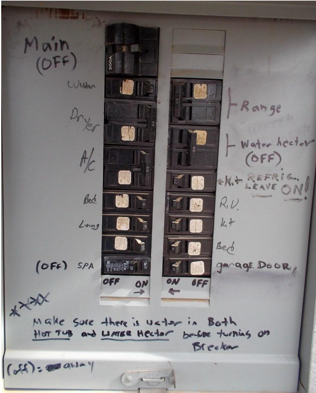
Figure 2. The switches which should be off when the house is not occupied are noted with (OFF). This includes the MAIN, Water Heater and the SPA. Note that the breaker on and off locations are mirror image for each side, i.e., OFF is always to outside.
