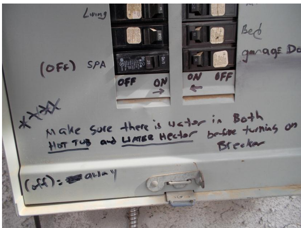
Figure 7. Once the hot tub is FULL of water, you can turn the SPA breaker on. WARNING – do not turn the SPA breaker on if the hot tub is not full of water.
